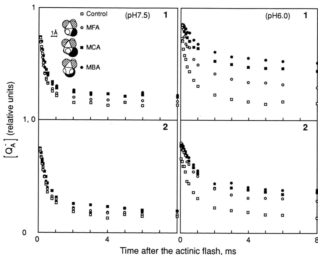
Fig. 2. [Q_A^-] decays in control and 100 mM monohalogenated acetate-treated spinach thylakoids after flash 1 and 2. See text for details.
