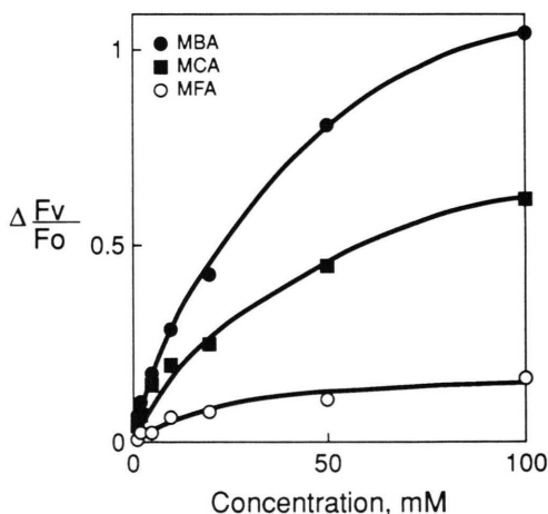
Fig. 1. Dependence of the change of variable Chl a fluorescence field, measured at 3 ms after the first actinic flash, as a function of concentration of monohalogenated acetates in spinach thylakoids at pH 6.0. See text for details.
